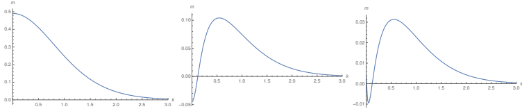
Figure: The constituent quark masses m_c(k) in the chiral limit m_0 = 0 , solutions of the mass gap equation, from left to right for the ground state vacuum and first two replicas.
