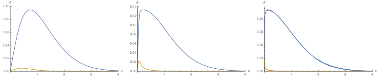
Figure: The J^{PC} = 1^{+-}, ^1P_1 normalized axial vector (A) radial wave functions \phi^+ (in blue) and \phi^- (in yellow), from left to right for the ground state vacuum and first two replicas, in dimensionless in units of K_0 = 1 .
