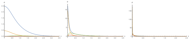
Figure: The J^{PC} = 1^{--}, {}^3P_1 normalized vector (V) radial wave functions \phi_0^+ (in blue), \phi_0^- (in yellow), \phi_2^+ (in green) and \phi_2^- (in red) from left to right for the ground state vacuum and first two replicas, in dimensionless in units of K_0 = 1 .
