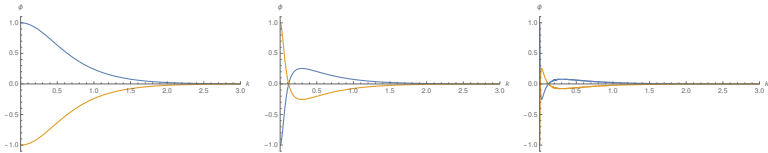
Figure: The J^{PC} = 0^{-+}, {}^1S_0 normalized pseudoscalar (P) radial wave functions \phi^+ (in blue) and \phi^- (in yellow), from left to right for the ground state vacuum and first two replicas, in dimensionless units of K_0 = 1 . Because the normalization diverges in the chiral limit, we arbitrarily normalize the wave functions with \phi(0) = 1 . Importantly, the wavefunctions \phi^\pm are identical to \pm \sin \varphi(k) = \pm m_c(k) / \sqrt{k + m_c(k)} as is easily verified from Fig. 5.
