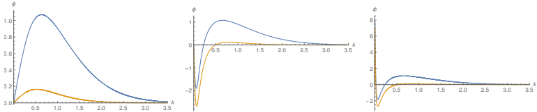
Figure: The J^{PC} = 0^{++}, {}^3P_0 normalized scalar (S) radial wave functions \phi^+ (in blue) and \phi^- (in yellow), from left to right for the ground state vacuum and first two replicas, in dimensionless in units of K_0 = 1 .
