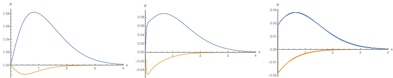
Figure: The J^{PC} = 1^{+-}, ^3P_1 normalized axial vector (A) radial wave functions \phi^+ (in blue) and \phi^- (in yellow), from left to right for the ground state vacuum and first two replicas, in dimensionless in units of K_0 = 1 .
