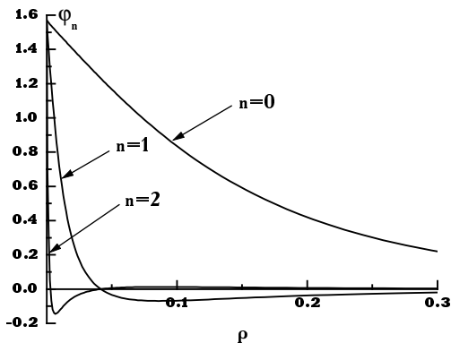
Figure: The first solution, \varphi_0(k) , of the mass gap equation, representing the vacuum |0\rangle and its two first two other solution, \varphi(k)_1 and \varphi(k)_2 for a linear confining potential [7, 4], corresponding to the truncated Coulomb gauge of QCD), computed in the chiral limit of m_q \rightarrow 0 .
