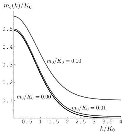
Figure: The dependence [3] of the constituent quark mass m_c(k) on the current quark mass m_0 .
