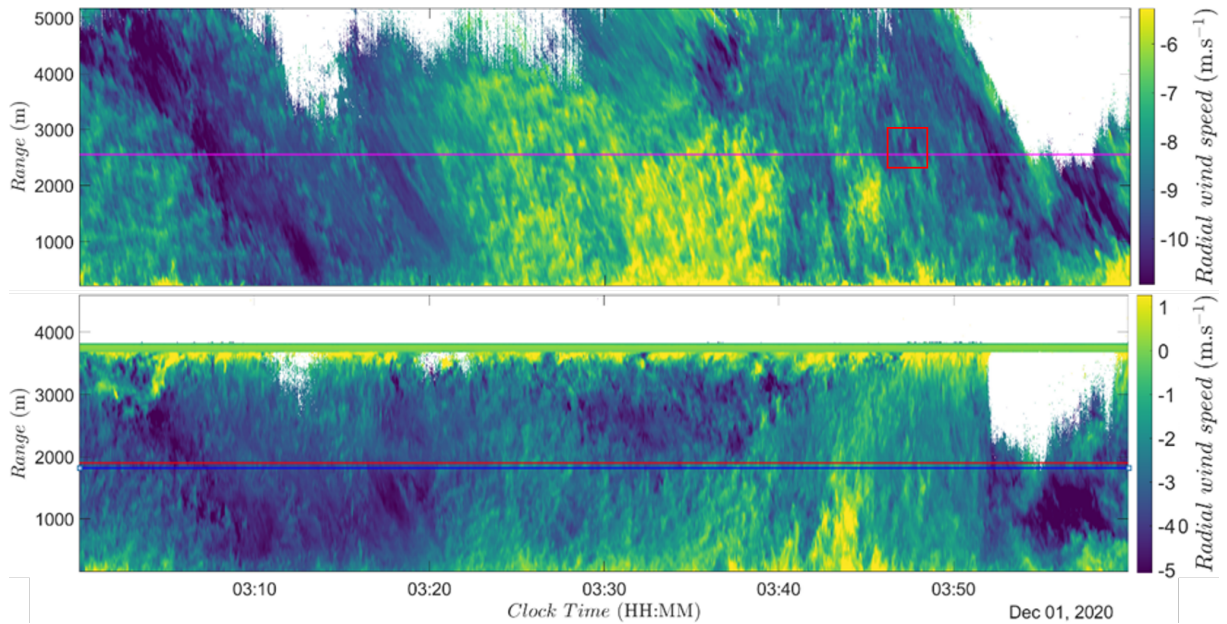
Figure 3. Spatiotemporal fluctuations of wind velocity recorded on 1 December 2020, 03:00 to 04:00 by (top) Donald and (bottom) Dolly. Intersection with other lidar(s) are indicated by colour horizontal lines.
