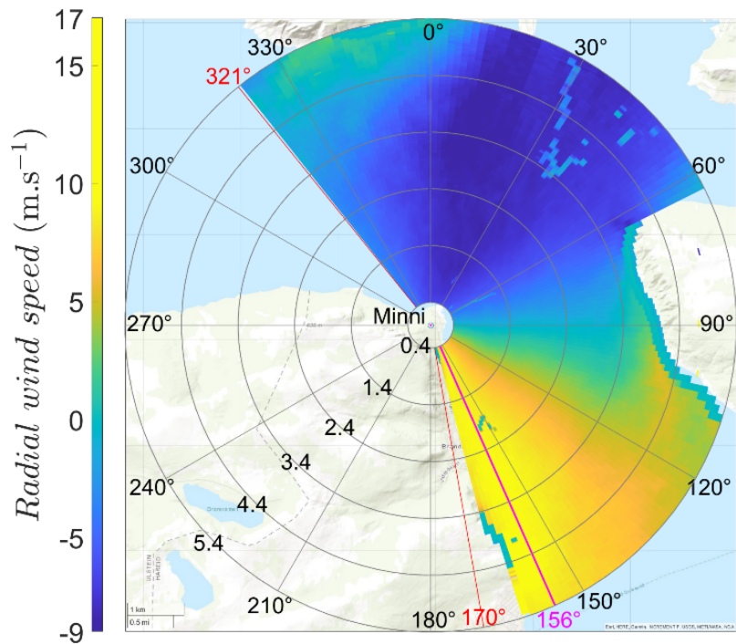
Figure 4. Mean of the along-beam wind velocity derived from PPI scans recorded on 1 December 2020, 03:00 to 04:00. Positive velocity is away from the lidar.
